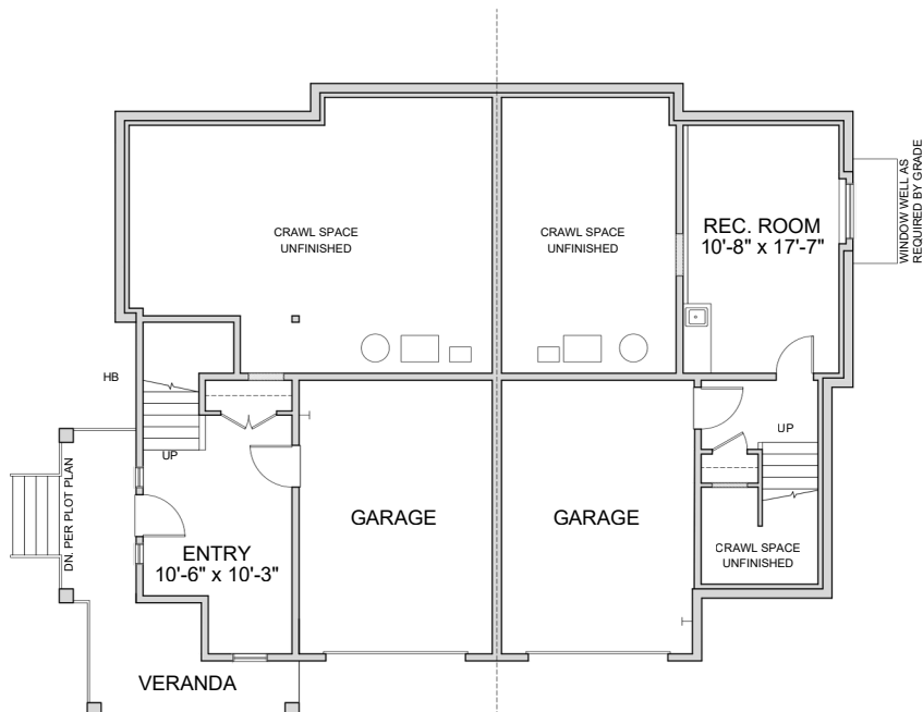
UNIT B: 958 SF
