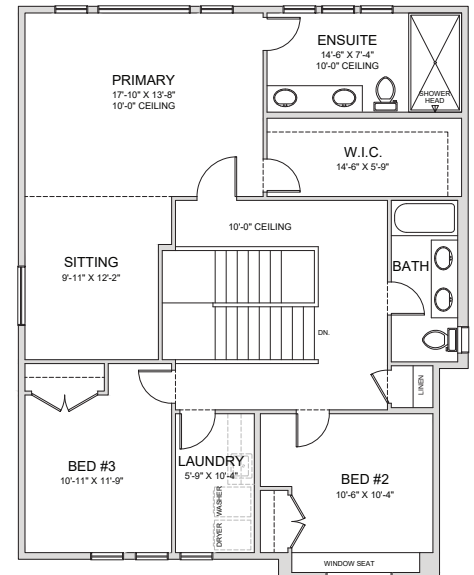
UPPER FLOOR - SITTING ROOM 1,292 SF
