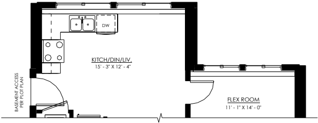
FINISHED DAYLIGHT BASEMENT w/1 BEDROOM SUITE
