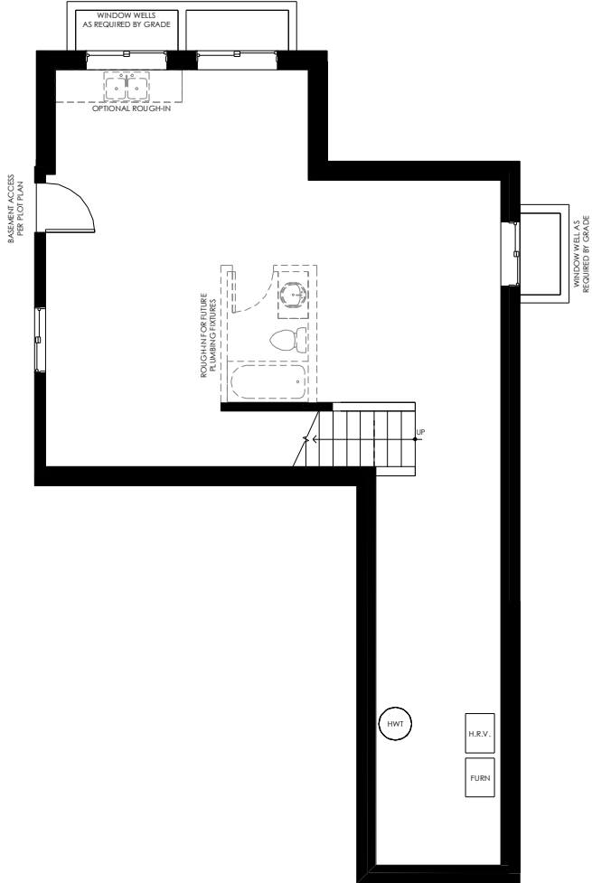
UNFINISHED BASEMENT
