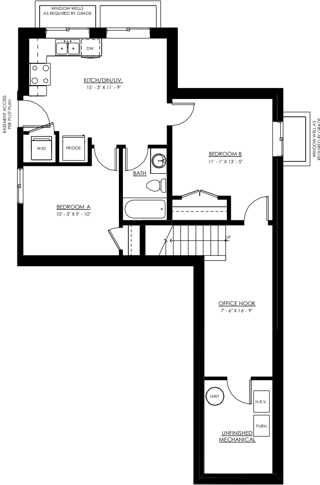
FINISHED BASEMENT w/2 BEDROOM SUITE SUITE AREA 633 SF BASEMENT AREA 946 SF
