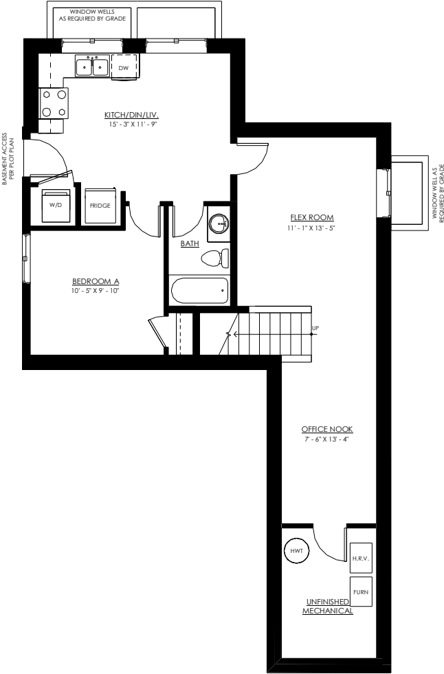
FINISHED BASEMENT w/1 BEDROOM SUITE SUITE AREA 444 SF BASEMENT AREA 946 SF
