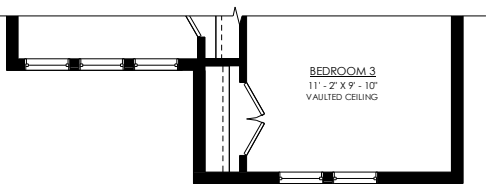
UPPER FLOOR BASED ON ASCOTT 'B'
