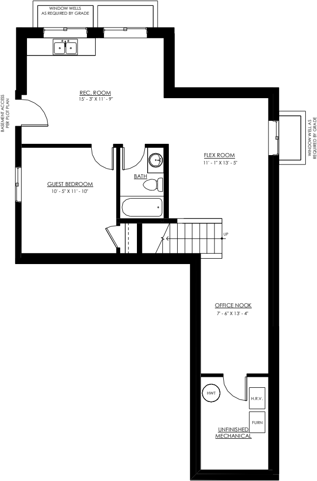
FINISHED BASEMENT BASEMENT AREA 946 SF
