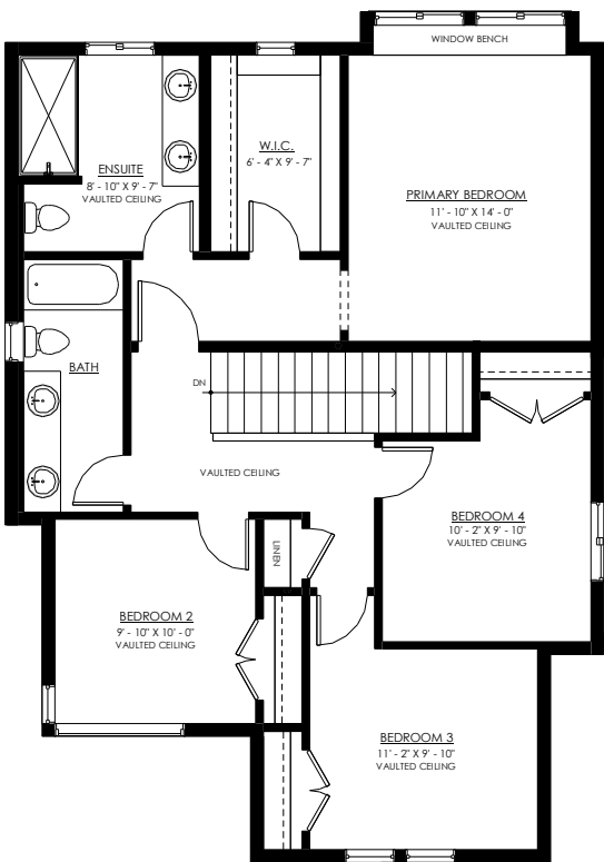
UPPER FLOOR - 4 BEDROOM BASED ON ASCOTT 'A'
